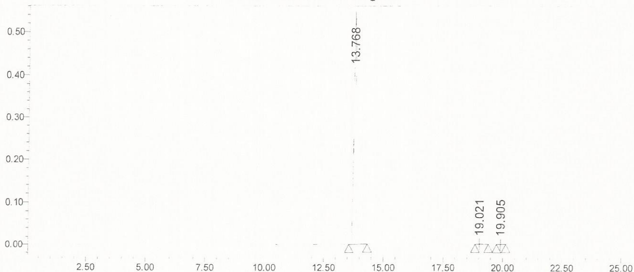
Auto-Scaled Chromatogram
